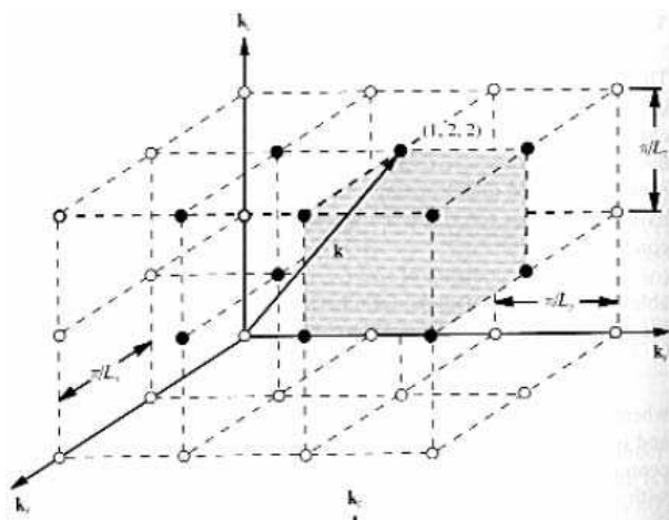
Figure 13: This figure shows a cube in k-space. The axes in k-space are k_x, k_y, k_z .
