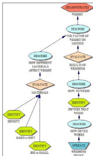
Figure 2 Content Hierarchy
